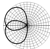
COL2 Max Radiation Pattern 120°
